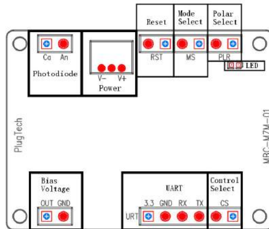
Figure 7. Assembly
