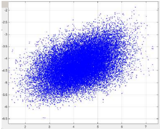
Figure 3. QPSK Constellation pattern (without controller)
