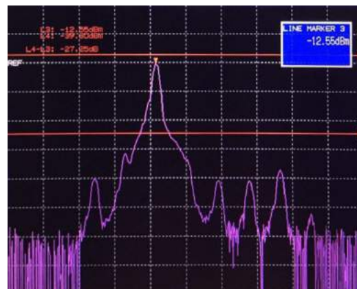
Figure 8. CS-SSB Spectrum
